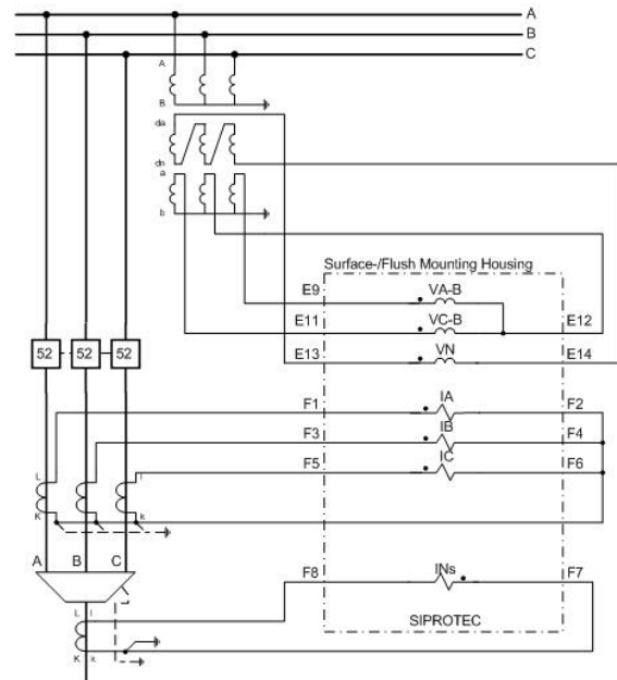
Fig.2: Connection diagram 7SK80
