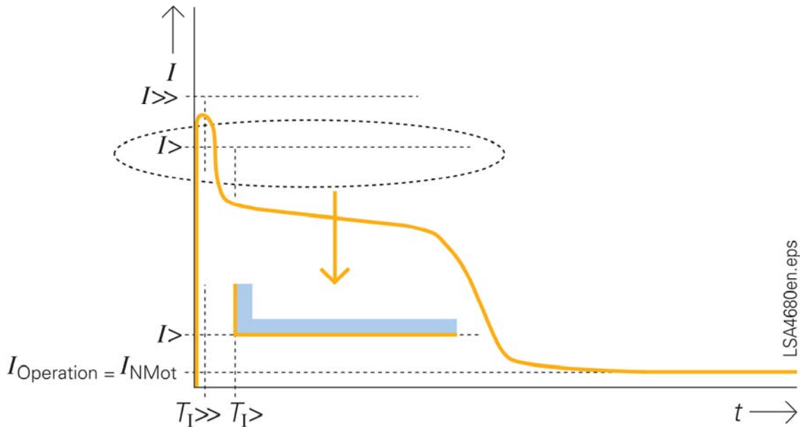
Fig.6: Reducing the time-overcurrent protection I > stage during rated operation
