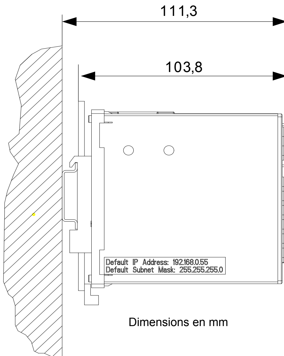
Figure 18-1 Dimensions
