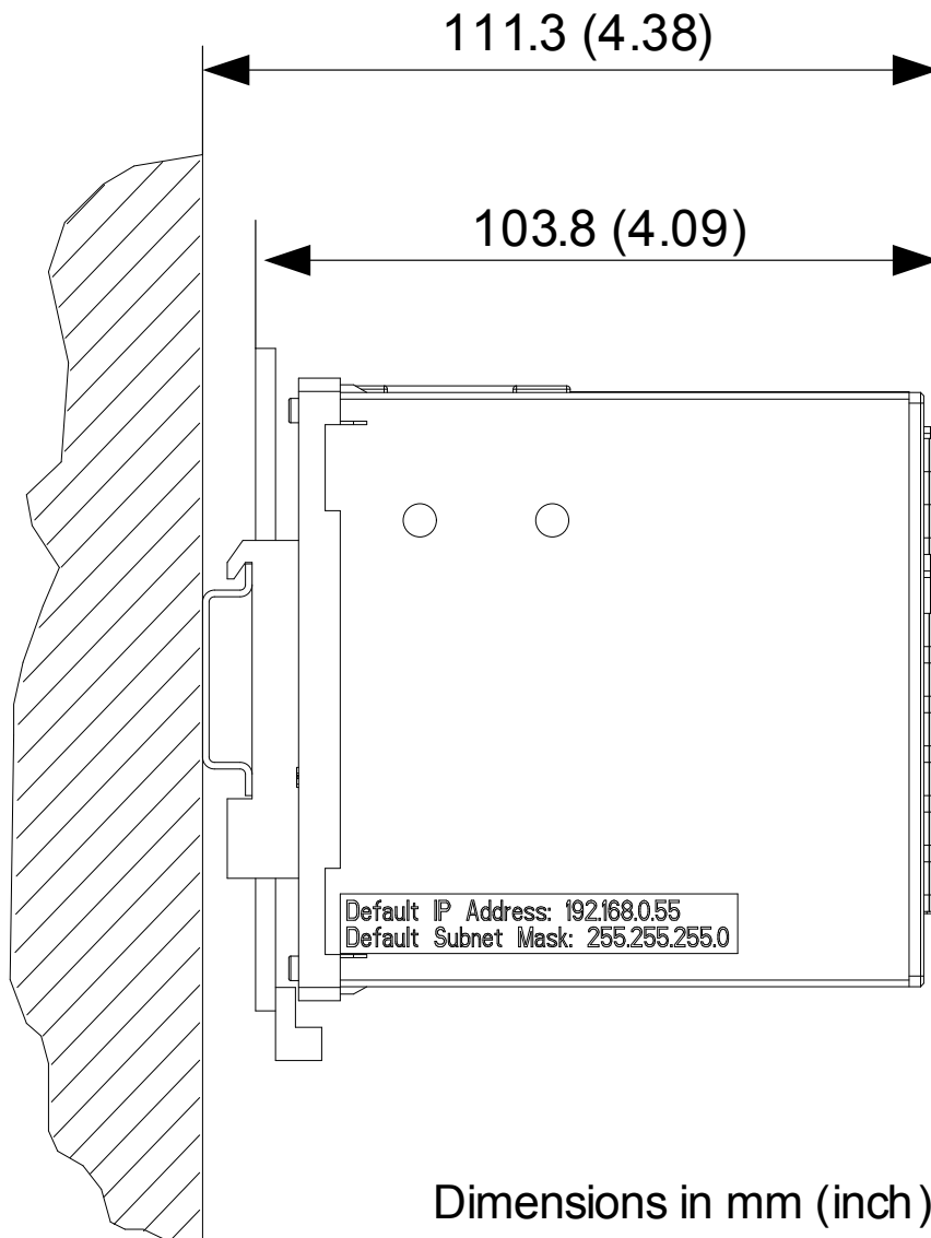
Figure 17-1 Dimensions
