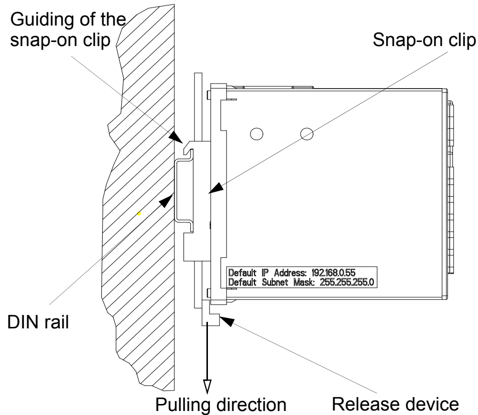
Figure 8-1 Mounting on a DIN rail
