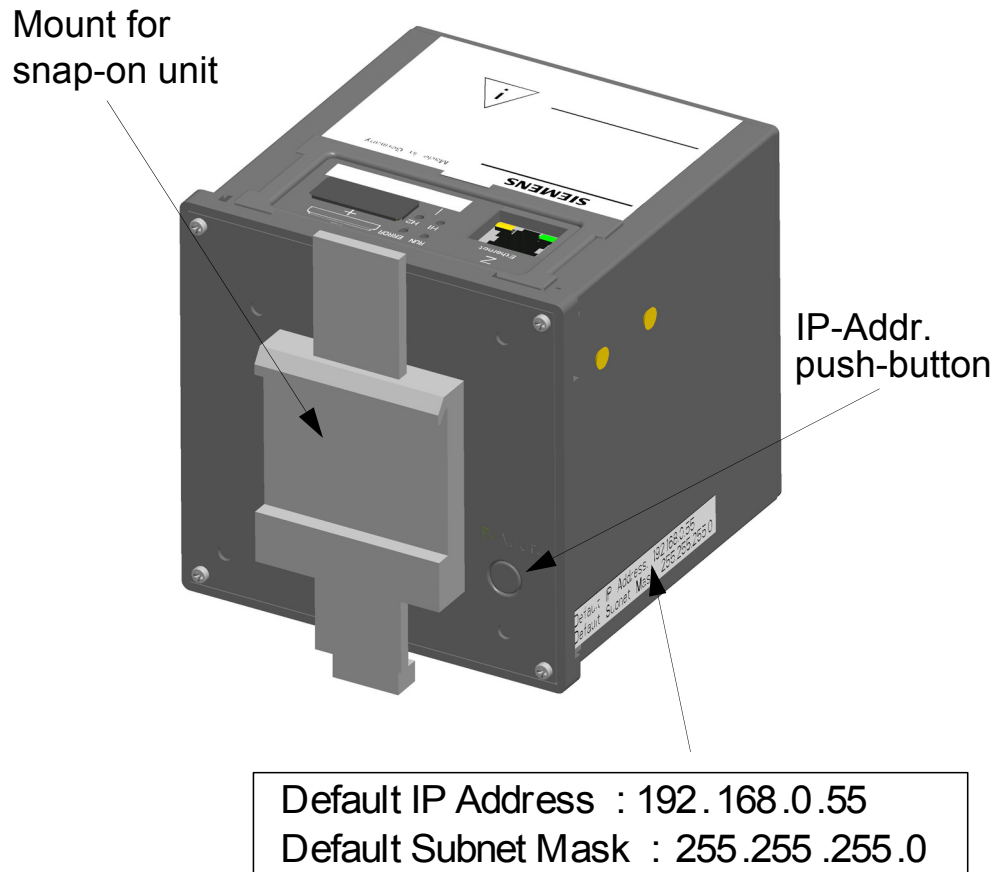
Figure 7-2 DIN Rail Side of SENTRON T 7KG966
