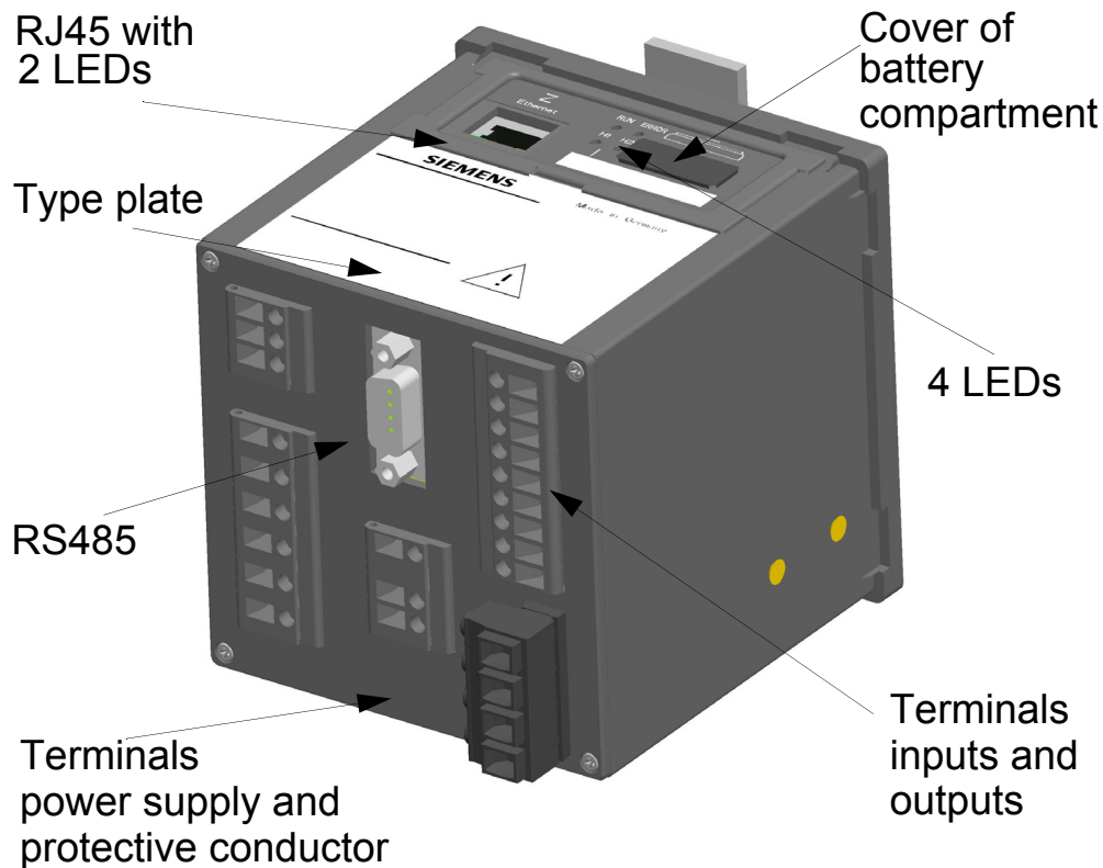
Figure 7-1 Terminal Side, SENTRON T 7KG966 with RS485
