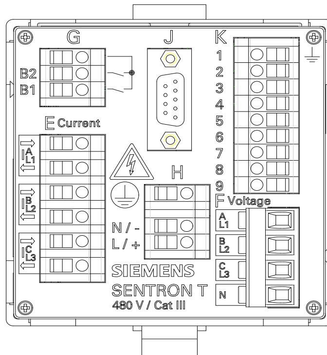
Figure 11-1 Terminals on the Terminal Side
