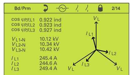
Fig. 13/10 Phasor diagram (SIMEAS P610)
