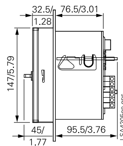
SIMEAS P6xx with transparent plastic facia IP54 Fig. 17/49
