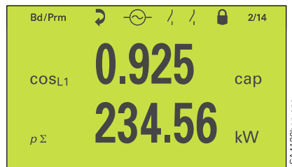
Fig. 13/4 2 measured values - digital (SIMEAS P610)
