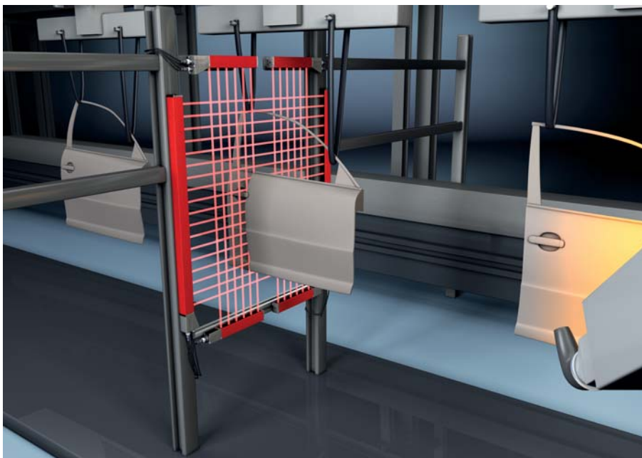
Figure 5.4: Contour measurement
