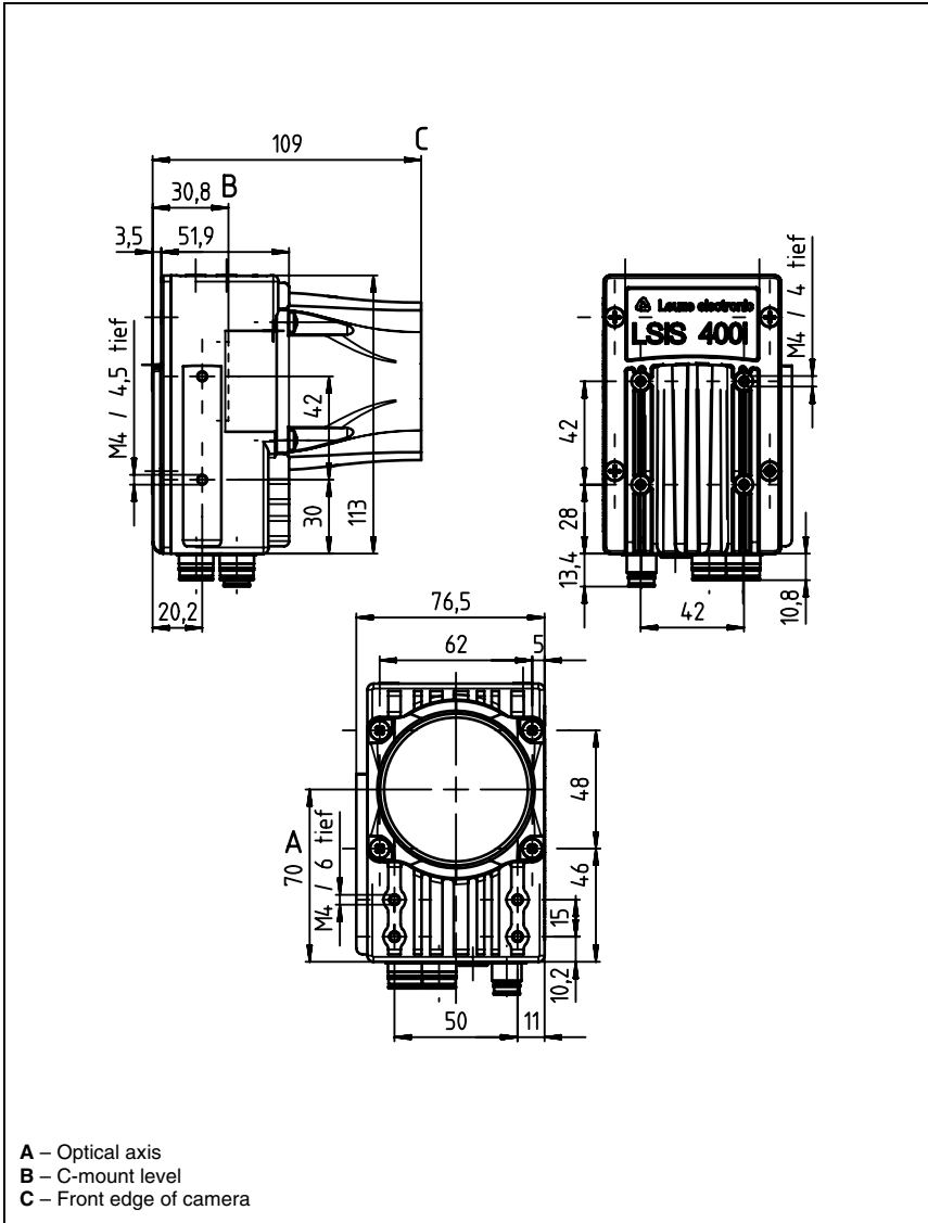
Figure 11.2: Dimensioned drawing of the LSIS 4xx i smart camera - devices for C-mount lenses
