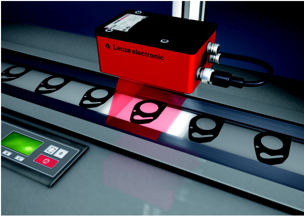
Figure 3.7: Application example - measurement of radii and roundness
