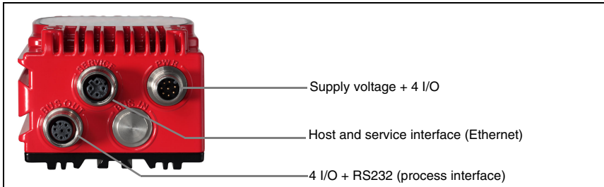
Figure 3.11: Stand-alone connection
