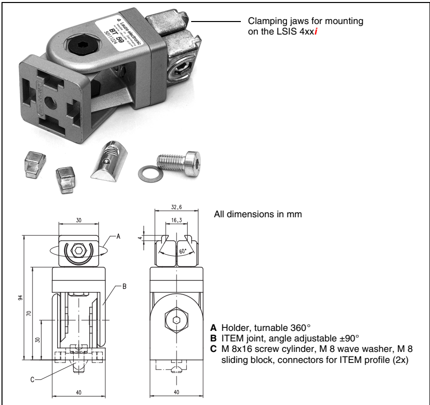
Figure 4.5: BT 59 mounting device
