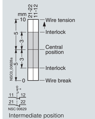
3SE7 160-1BD00
