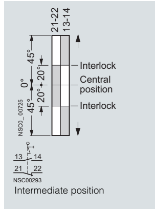
3SE7 160-1BD00
